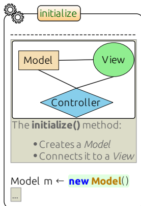
Fig. 5. An early prototype of our rich comment editor supporting diagrams.
