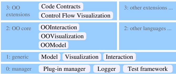
Fig. 9. The different layers and plug-ins of Envision’s architecture.
