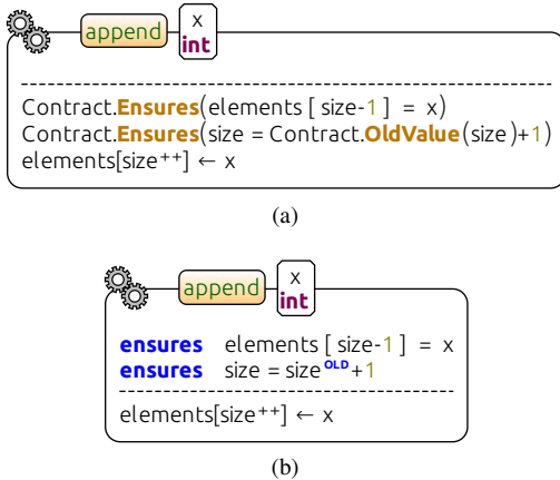
Fig. 4. (a) A method that appends an element to a list using .NET Code Contracts to specify postconditions and (b) the same method with custom visualizations for the contract method calls. Both forms are editable.
