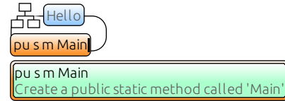
Fig. 8. An abbreviated command in a prompt invoked on a class object.
