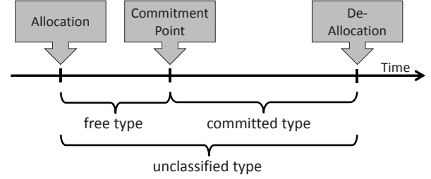
Figure 2. Newly-allocated objects have a free type until they reach their commitment point, when the type changes to a committed type for the rest of the object’s lifetime. Unclassified types subsume free and committed types.
