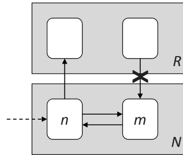
Figure 3. Heap structure for the execution of a new-expression that takes only committed arguments. Objects are depicted by rounded boxes; references in fields and on the stack are depicted by solid and dashed arrows, respectively. The set N contains the objects created during the execution of the new-expression; the set R contains the (committed) objects reachable from the new-expression’s arguments. Here, both objects in N are free until the new-expression terminates and, therefore, cannot be referred to by the committed objects in R .
